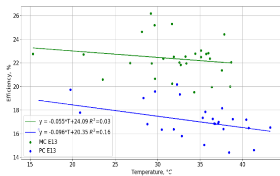
Figure 3. Actual efficiency of E13-oriented panels with respect to the maximum temperature of the panels surface, in September 2020.
