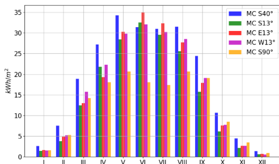
Figure 1. Energy produced by monocrystal panels in 2020, shown by month.
