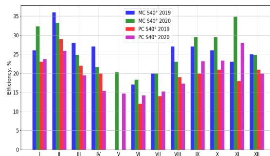
Figure 5. Actual efficiency of S40-oriented panels by month in 2019 and 2020.
