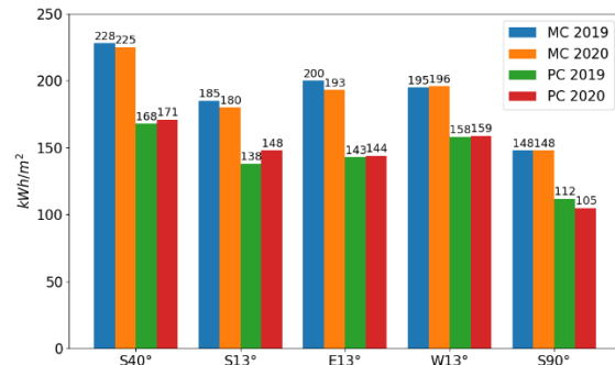
Figure 2. Total energy produced by varied-oriented panels during 2019 and 2020.
