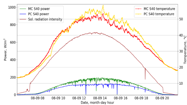
Figure 4. S40 panels' surface temperatures, solar radiation intensity on a horizontal surface and the panels' power output on a sunny August day.
